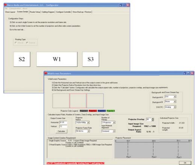
Configurator GUI
